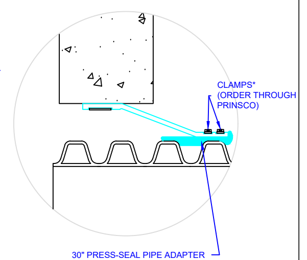
A 120 GASKET DETAIL SCALE: NTS
